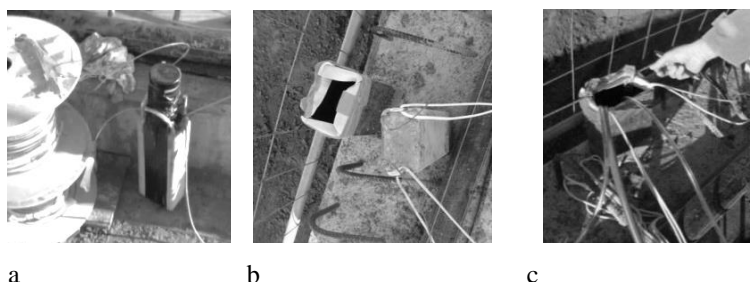
Figure 3. Pictures of the installation details of OV2 and OV3: a) metal weight for OV2; b) metal weight for OV3; c) OV3 before grouting
