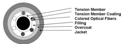
Figure 1. Cross section cementys sensoLux™ (Cementys, 2014)
