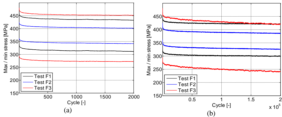
Fig. 4. Evolution of \sigma_{\max} and \sigma_{\min} versus cycles for (a) 2000 and (b) 200000 cycles.
