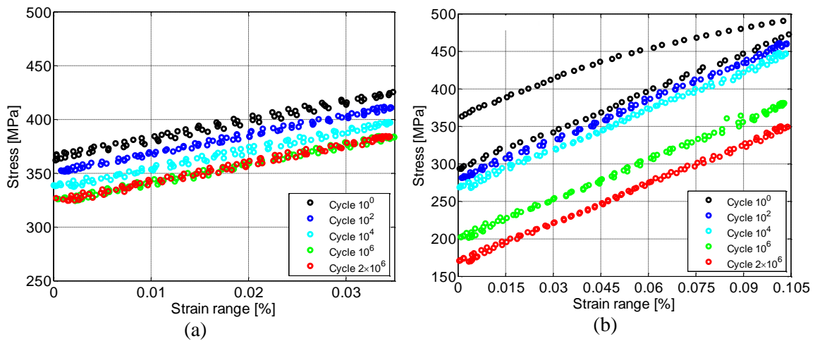
Fig. 3. SMA (activated) stress-strain behavior under fatigue loading for (a) Specimen F2 with \Delta\varepsilon_0 = 0.035\% , (b) Specimen F3 with \Delta\varepsilon_0 = 0.105\% .
