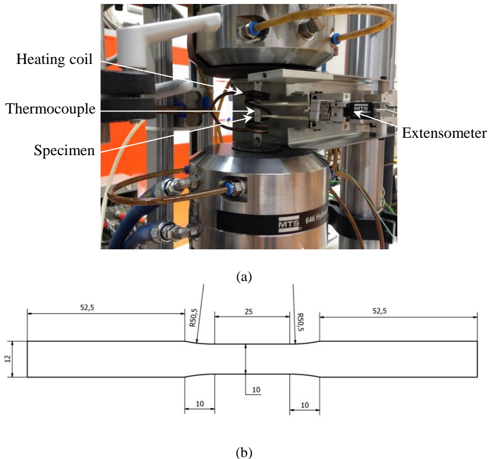
Fig. 1. (a) Testing equipment, (b) dog bone specimens with 1.5mm thickness (dimensions in mm).
