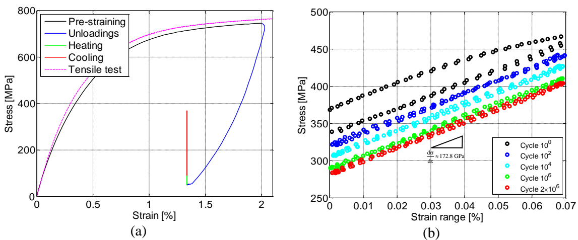
Fig. 2. Specimen F1. (a) stress-strain curve during activation process, (b) SMA (activated) stress-strain behavior under fatigue loading with \Delta\epsilon_0 = 0.070\% .
