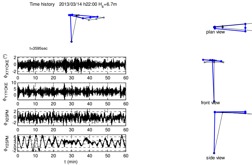
Figure 17. Time history inclinometers and position of the system, storm of 2013/03/14, h22.
