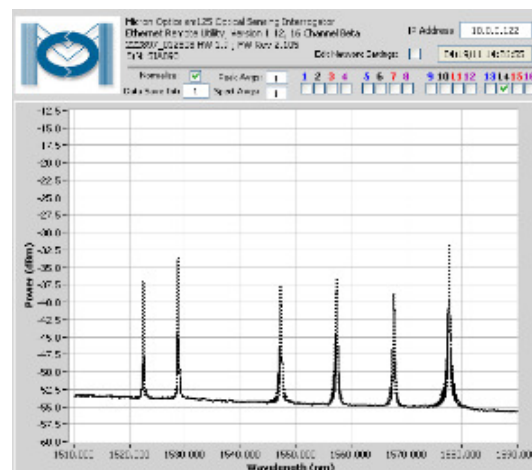
Figure 6. Control unit channel #14; 1519_T_8_3, 1526_T_8_6, 1542_S_8_1, 1552_S_8_2, 1562_S_8_4, 1572_S_8_5.
